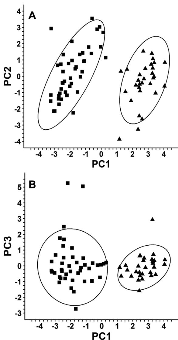
Fig. 1. PCA of the proportional morphometrics of C. pennsylvanicus (squares) and F. subsericea workers (triangles). Panel A depicts PC axis 1 (48.5% of variation) versus PC axis 2 (17.9%), whereas panel B depicts PC axis 1 versus PC axis 3 (14.3%). The ellipses depict the 95% confidence interval for the location of each group centroid.
