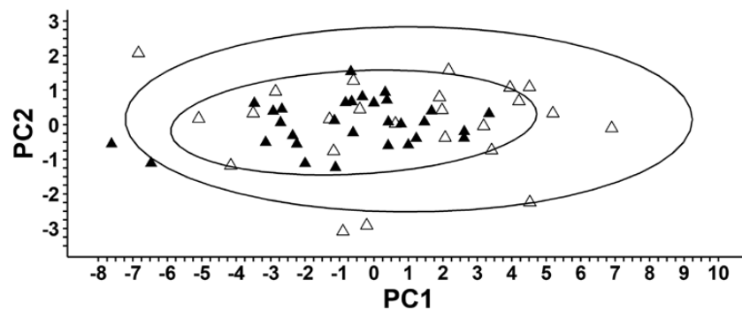
Fig. 4. PCA of the absolute morphometrics of F. subsericea workers that exhibit swimming (filled triangles) or walking (hollow triangles) behavior during aquatic locomotion. The ordination depicts PC axis 1 (73% of variation) versus PC axis 2 (7%). The ellipses depict the 95% confidence interval for the location of each group centroid.
